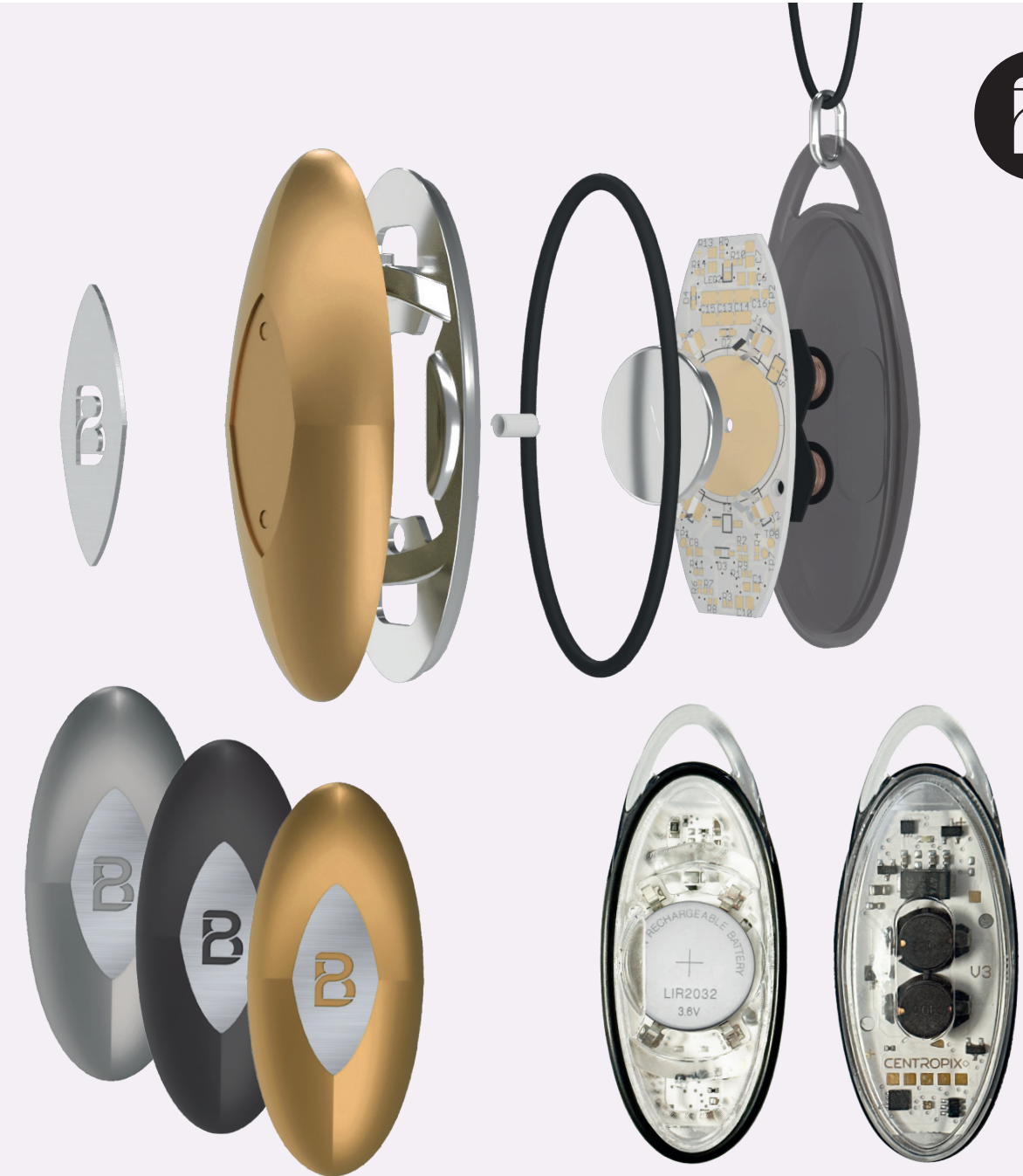
Demonstration model made of clear plastic (Left: front and open / Right: back)
